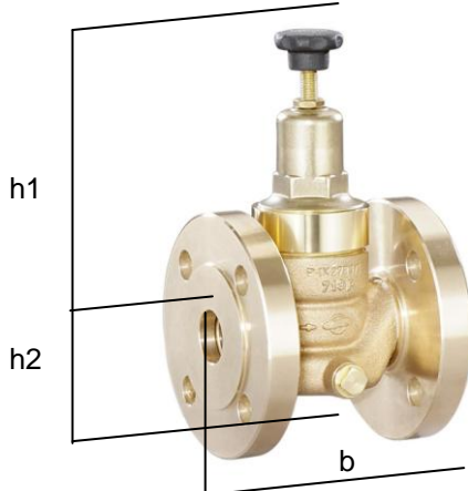
DN 15 - DN 32
