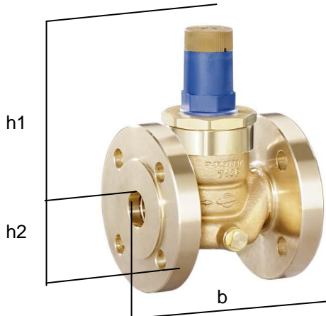
DN 15 - DN 32
